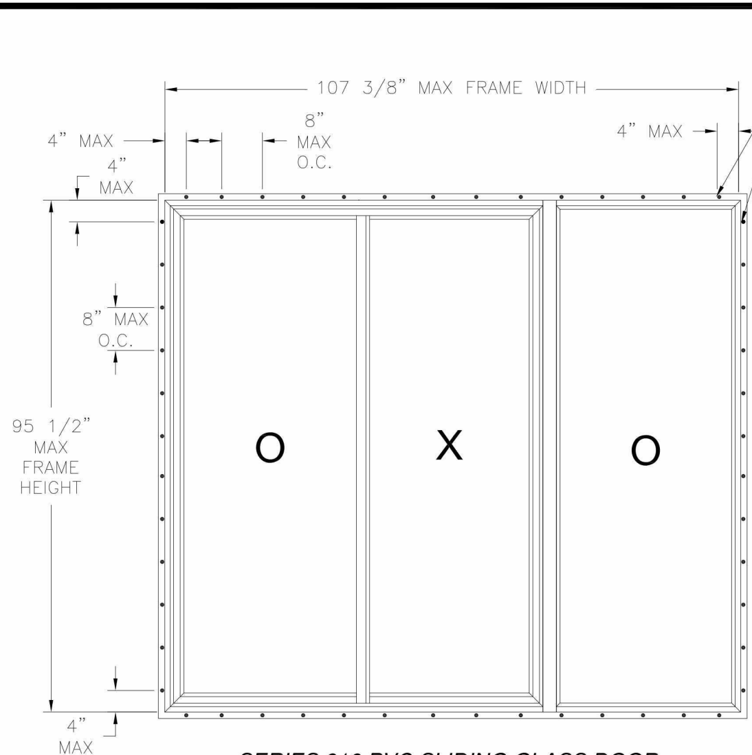
SERIES 910 PVC SLIDING GLASS DOOR EXTERIOR VIEW FIN INSTALLATION
