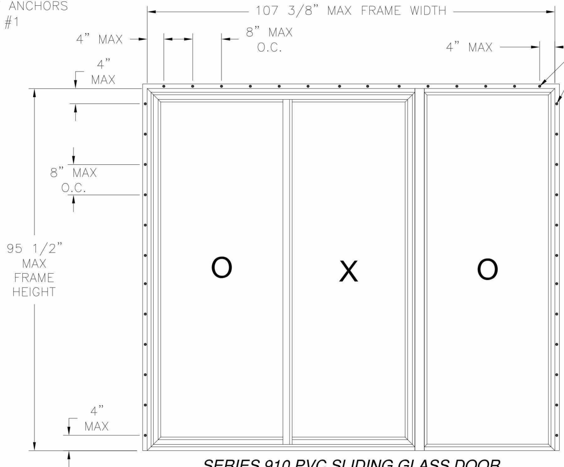
SERIES 910 PVC SLIDING GLASS DOOR EXTERIOR VIEW FIN INSTALLATION NO SILL ANCHORS
